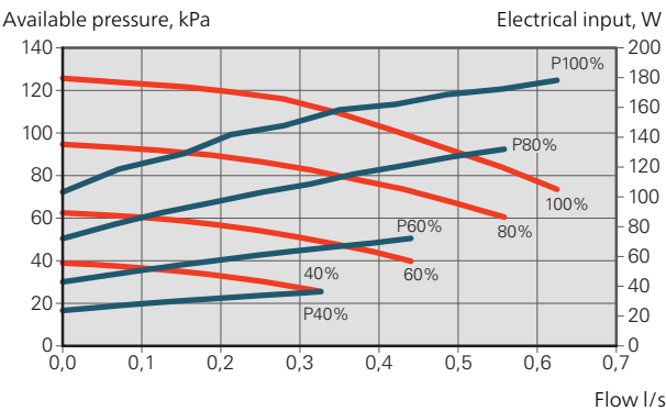
S1155 12 kW
