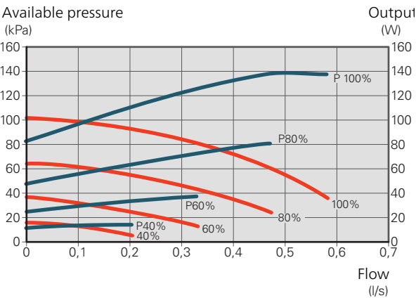
S1155 12 kW
